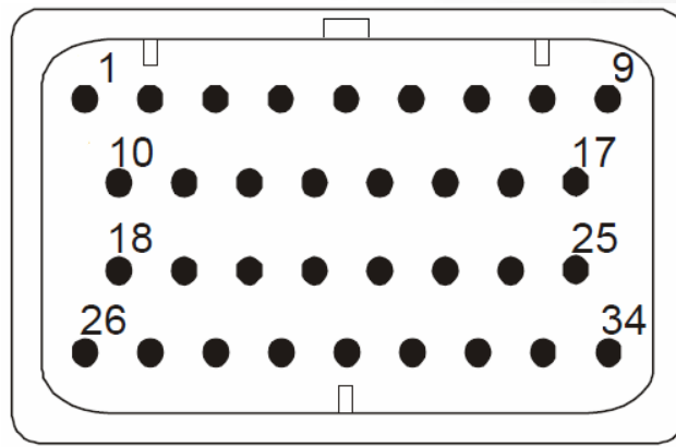
Mating Connector - 4-1437290-0
